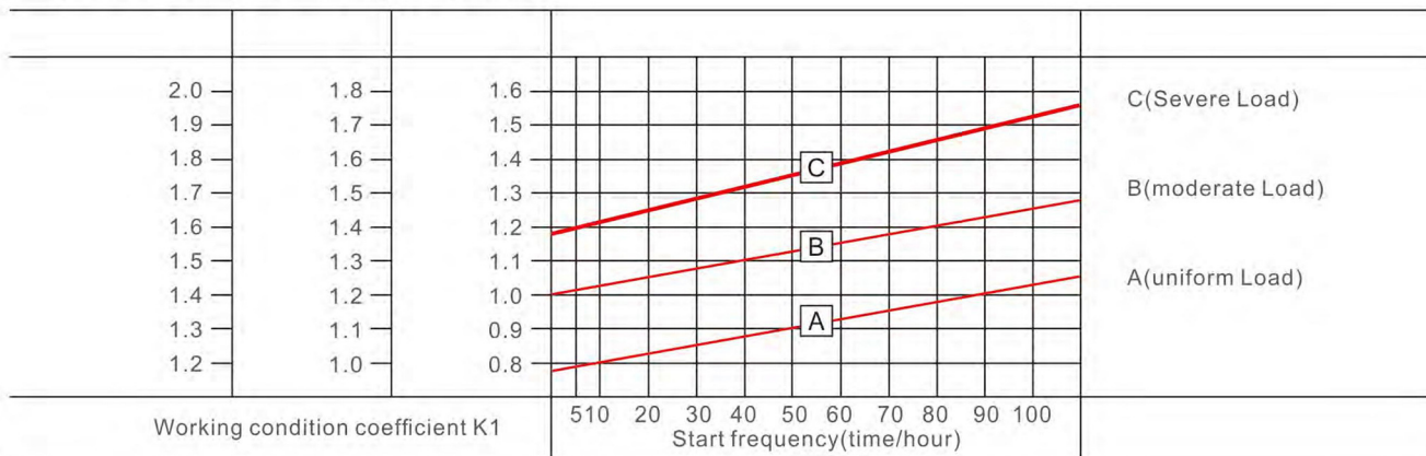
Diagram 1 working condition coefficient K1
